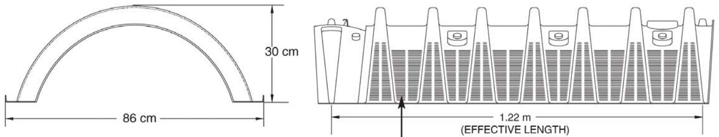
Sidewall louvers allow infiltration to sidewall of trench
